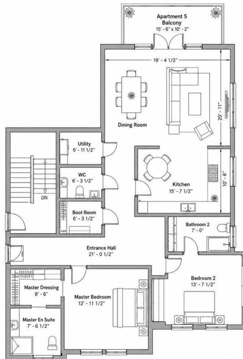
APARTMENT 5 – GREEN FLOOR PLAN
